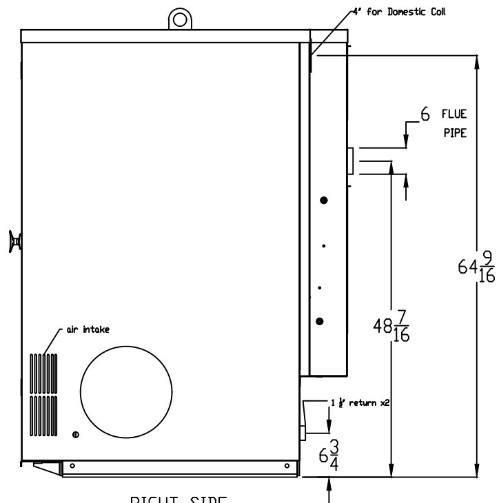
RIGHT SIDE
